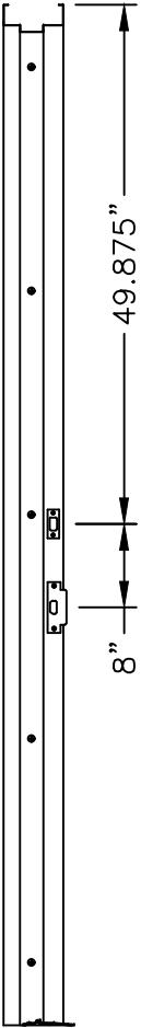
STRIKE PLATE LOCATIONS 2" HEAD
